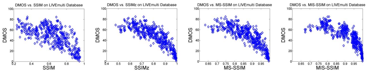
Fig. 7. Scatter plots of DMOS vs. SSIM, SSIMz, MS-SSIM and the proposed MIS-SSIM metrics on the LIVE multiply distortion database.
