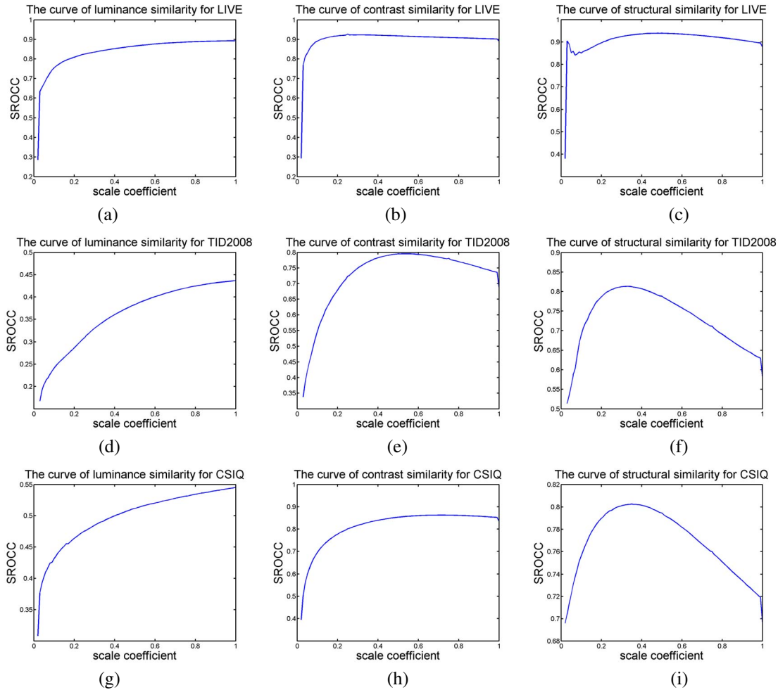
Fig. 1. The changing of curve of luminance, contrast, structural similarities under different scale coefficients for (a)-(c): LIVE database; (d)-(f): TID2008 database; (g)-(i): CSIQ database.
